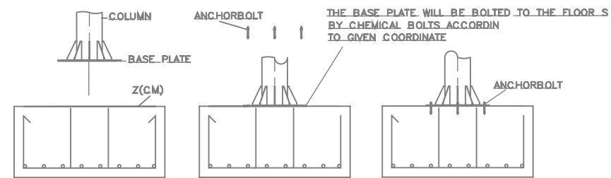
Column Installation Detail
